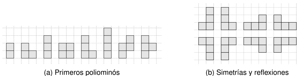
Figura 11.4: Poliomínos
